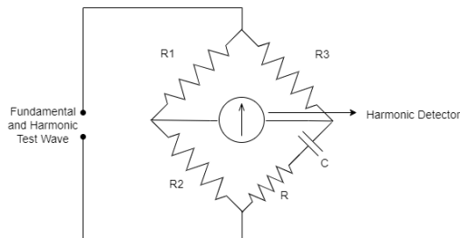
Fig. Resonance Bridge Circuit
