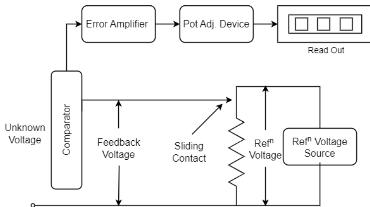
Fig: Servo Pot type DVM
