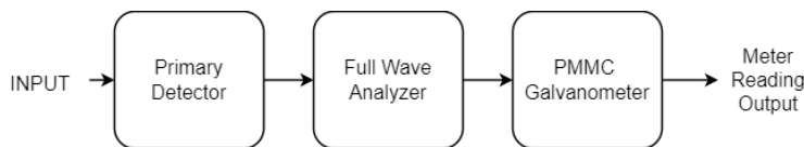
Fig: Basic Wave Analyzer
