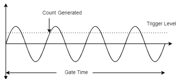
Fig: Basic concept of a frequency counter
