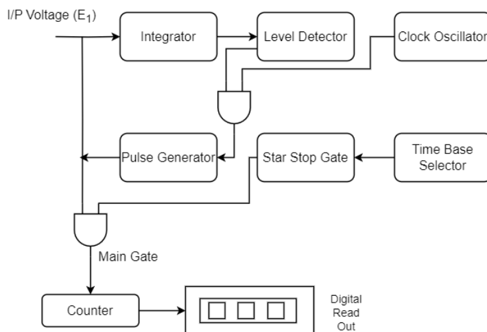
Fig: Integrating type DVM
