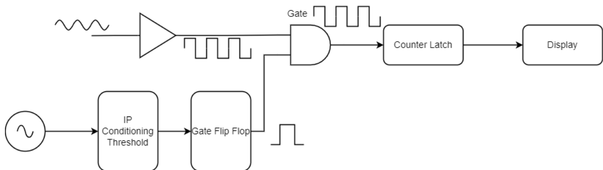
Fig: Frequency Counter
