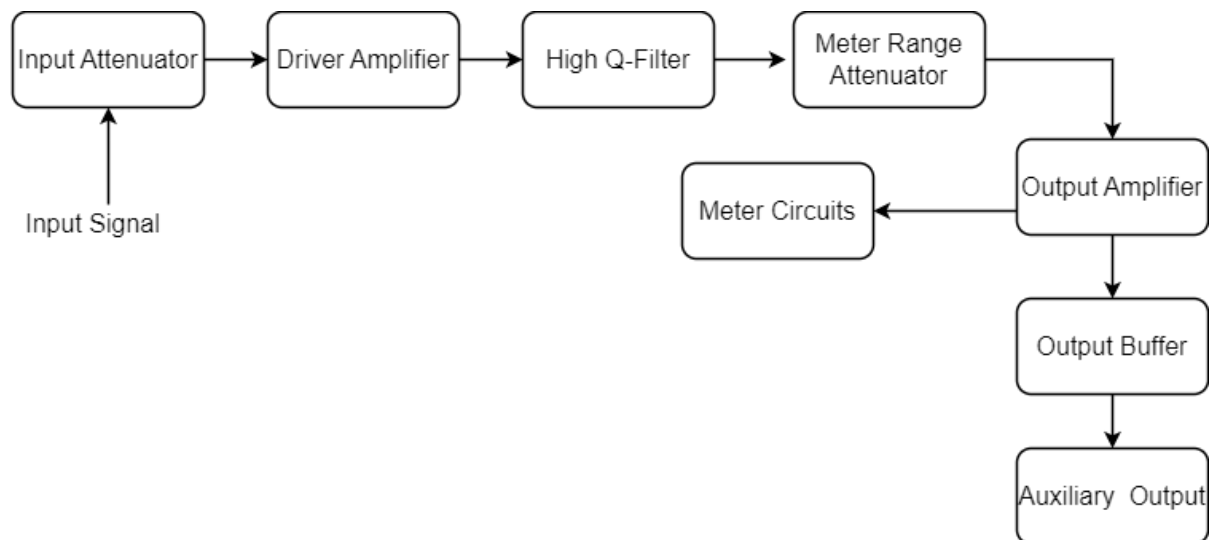
Fig: Frequency Selective Wave Analyzer
